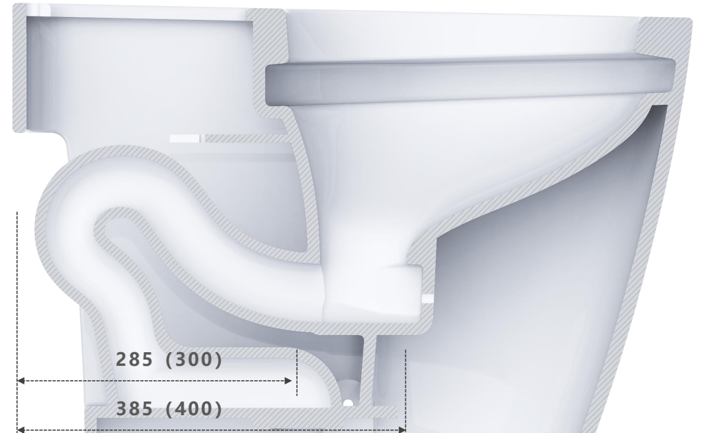
Adaptive on-floor drainage ceramic platform
