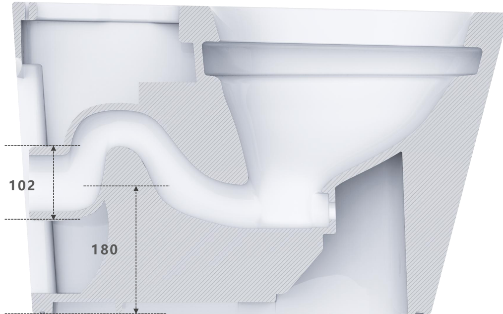
Adapted in-wall drainage ceramic platform
